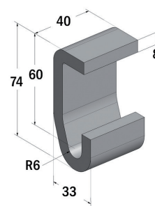
Support Bracket
