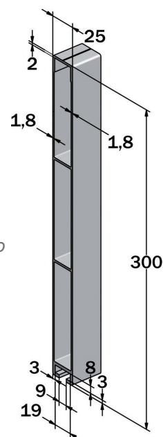
Without protective strip
