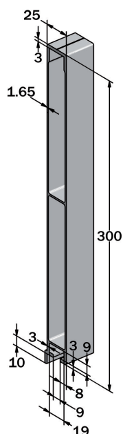
With protective strip
